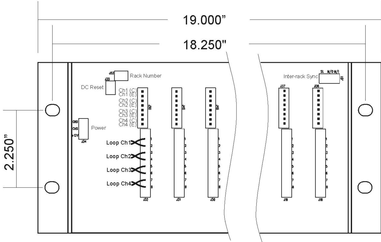
Rear View of Card Rack
